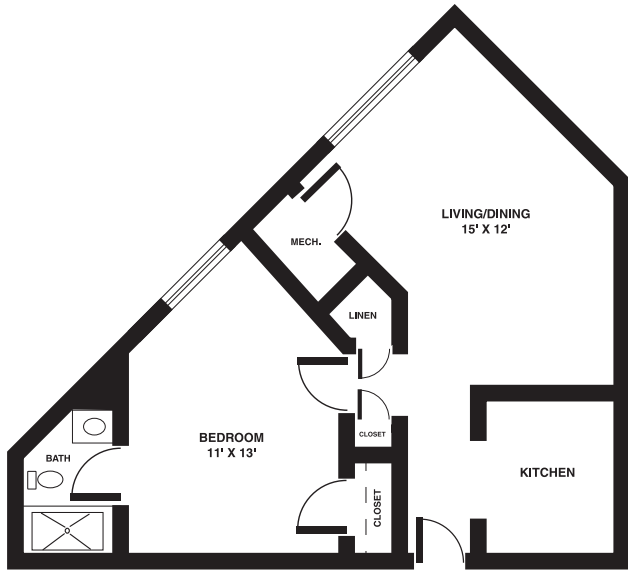
One-Bedroom
